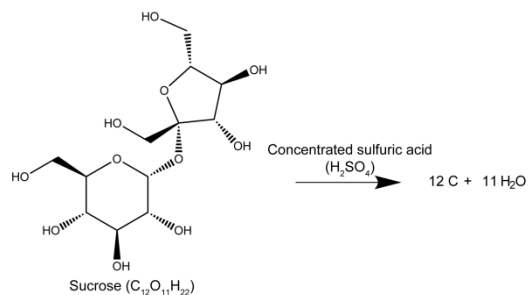
Figure 1. Formula of the bottom-up CQD synthesis mediated by dehydration of sucrose.
