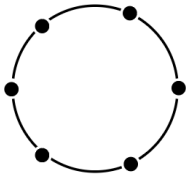
C_n (n \geq 6) n = \infty 即为无限路[5]
