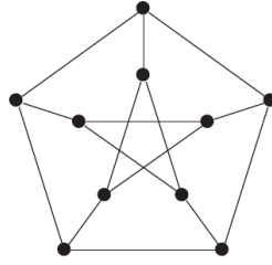
Petersen 图[5]
