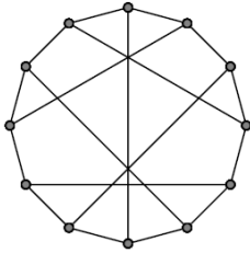
Triplex图[6]
